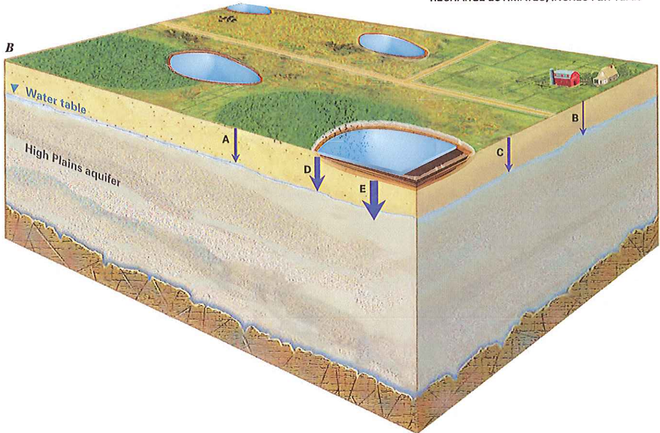
Figure 6. A, The recharge estimates listed in appendix 3 are summarized for each recharge setting (A–E); they generally indicate larger recharge rates beneath playas than beneath interplaya settings (note: x-axis is logarithmic). The size of arrows in (B) shows relative magnitude of recharge rates, which are approximations based on reported values and locations. Letters A–E refer to recharge settings lettered similarly in figure parts A and B.
